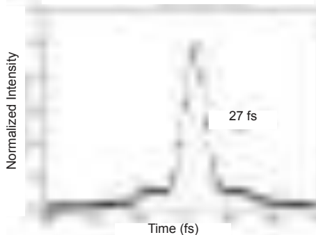
Fig. 2 Measured autocorrelation trace of the pulse
